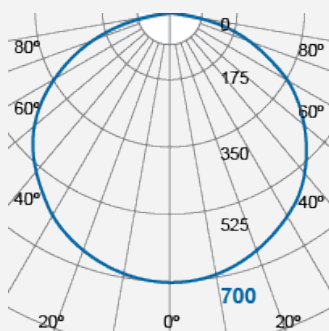
Integrated LED Luminaire F61500SM
