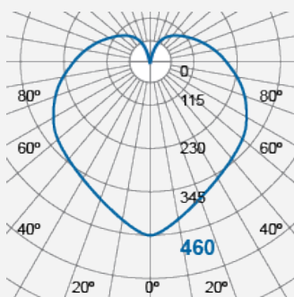
Integrated LED Luminaire FOB60900v0-pl
