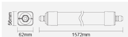
Integrated LED Luminaire FOB61100v0-pl
