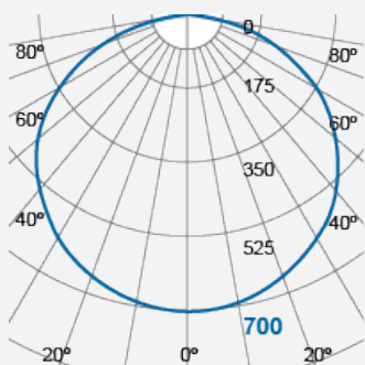
Integrated LED Luminaire FOB61500v0-pl
