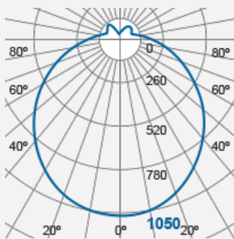
Integrated LED Luminaire FIB70200v0-pl
