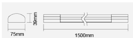
Integrated LED Luminaire FIB70200v0-pl
