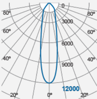
Luminaire with LED Module TECOH® RDx RD0343M (1400mA) F25349TK-25 °
