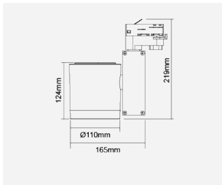
Luminaire with LED Module TECOH® RDx RD0343M (1400mA) F25349TK-25 °
