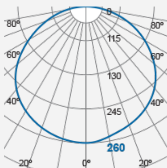
Integrated LED Luminaire F29000SM-3000K
