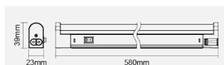
Integrated LED Luminaire F29000SM-3000K
