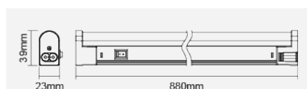
Integrated LED Luminaire F29100SM-3000K
