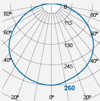
Integrated LED Luminaire FIB71500v0-3000K
