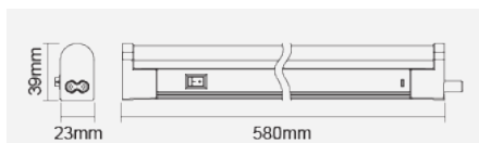
Integrated LED Luminaire FIB71500v0-3000K
