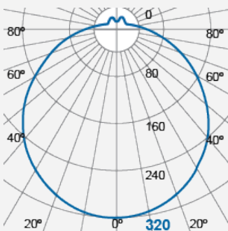
Integrated LED Luminaire FCL53600v0-em
