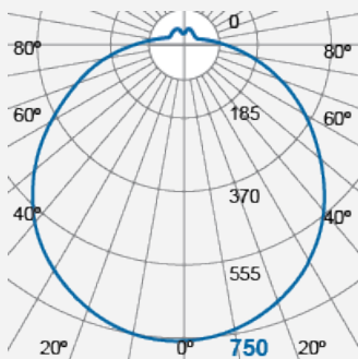
Integrated LED Luminaire FCL63300v0-ms
