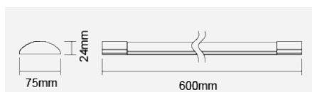
Integrated LED Luminaire FIB70500v1
