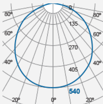
Integrated LED Luminaire FIB70500v1
