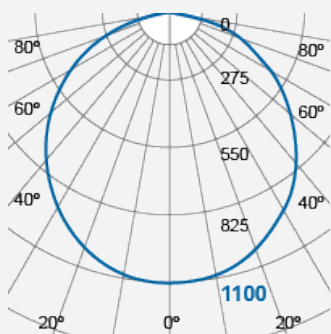
Integrated LED Luminaire FIB70700v0
