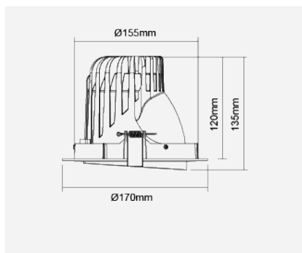
Luminaire with LED Module TECOH® RDx RD0343M (1050mA) F28249RC-35 °
