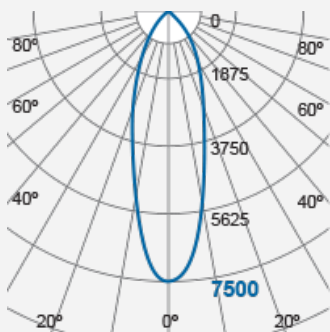
Luminaire with LED Module TECOH® RDx RD0343M (1050mA) F28249RC-35 °
