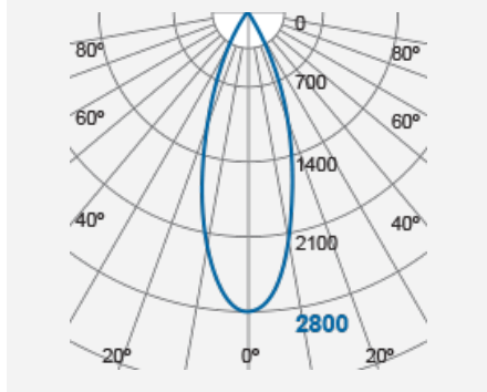
Luminaire with LED Module TECOH® MHx MH0219 (500mA) F51548RC-35 °
