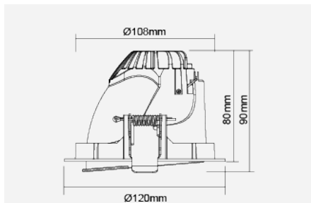
Luminaire with LED Module TECOH® MHx MH0219 (500mA) F51548RC-35 °
