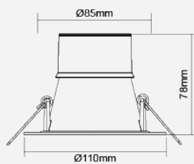
Integrated LED Luminaire F26400RC
