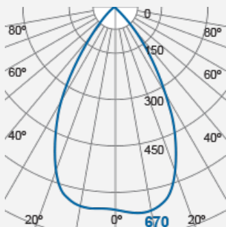
Integrated LED Luminaire F26400RC
