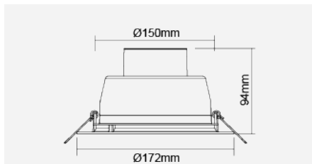
Integrated LED Luminaire F54200RC-d
