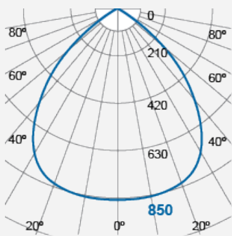
Integrated LED Luminaire F54200RC-d
