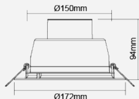
Integrated LED Luminaire F54700RC-d
