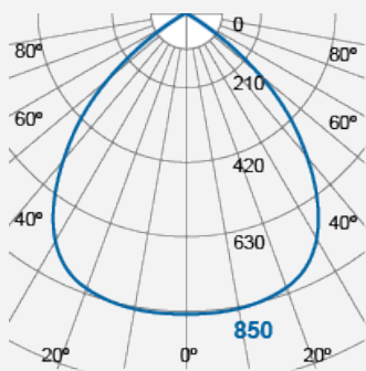
Integrated LED Luminaire F54700RC-d
