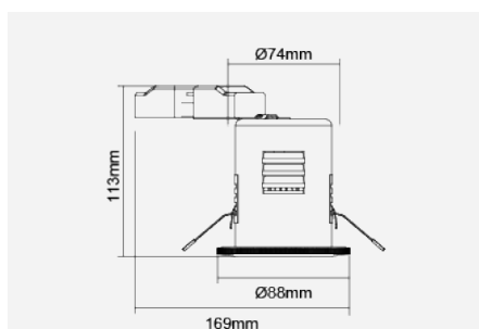
Luminaire with LED Light Engine TECOH® THx TH0106d
