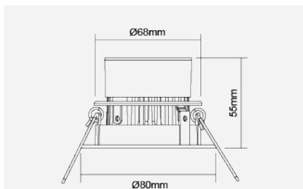
Integrated LED Luminaire F28100RC-dBT-24 °
