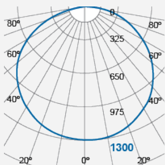
Integrated LED Luminaire FOB61500v1-pl
