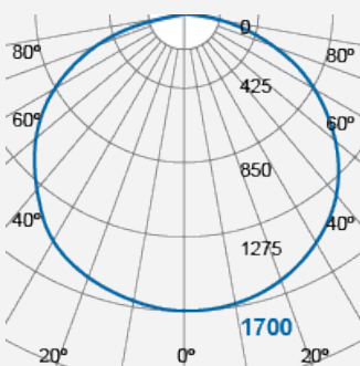
Integrated LED Luminaire FOB61600v1-pl
