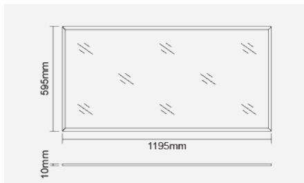
Integrated LED Luminaire F53800RCv1
