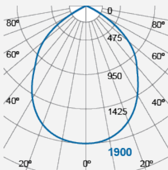
Integrated LED Luminaire F54300RCv1
